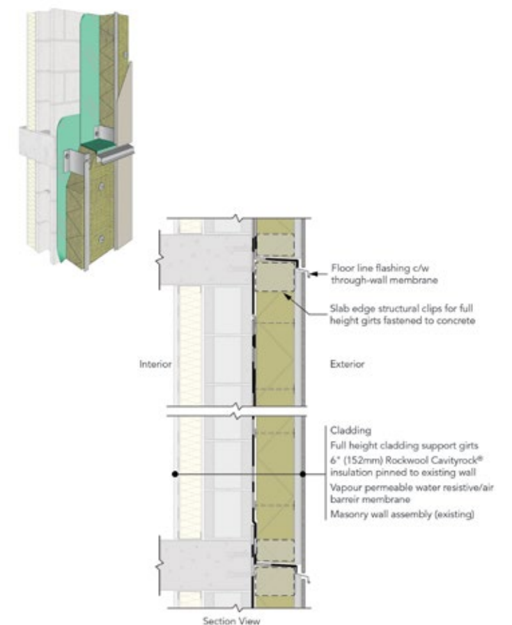
Figure 2: ROCKWOOL Cavityrock between a Z-girt clip system, installed over an existing CMU structure, attached through the concrete slab
