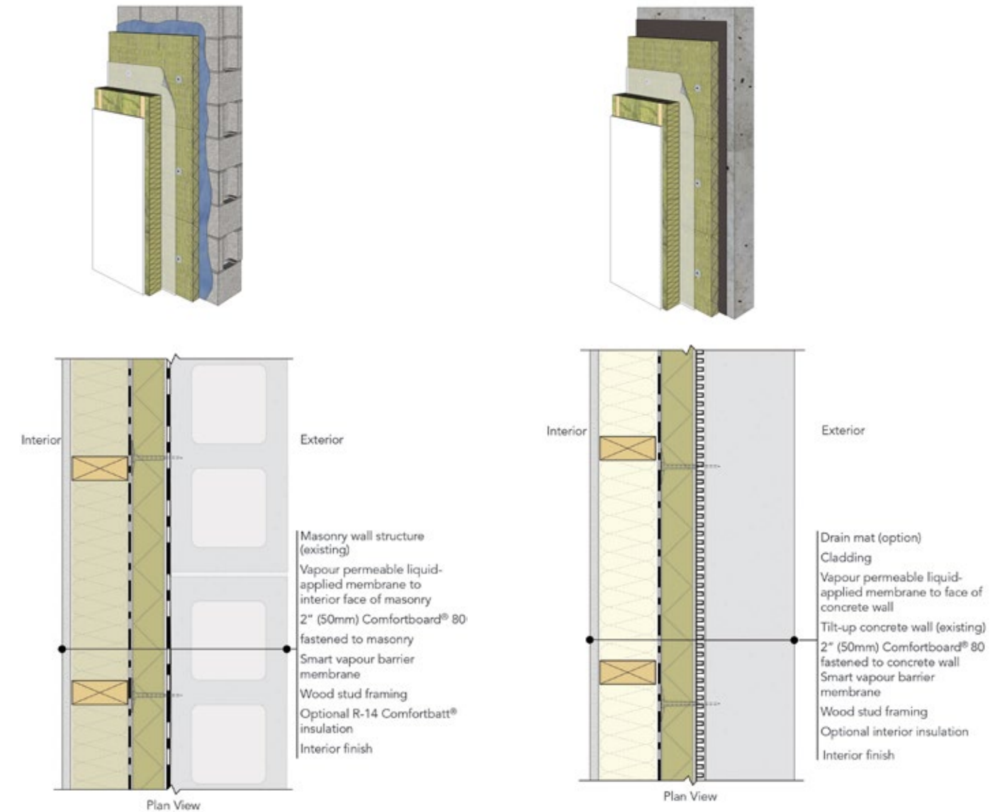
Figure 8: ROCKWOOL Comfortboard installed on the interior of an existing concrete tilt-up construction, with optional batt insulation installed between a wood frame
