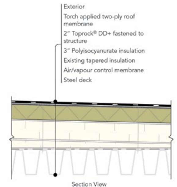
Figure 11: ROCKWOOL Toprock DD Plus installed on top of an existing roof structure, using a torch applied roof membrane
